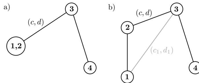
Figure 3.3: An example of a merge operation in the graph being undone for the tree. a) The initial situation on the higher level. b) The tree after the merge operation is undone. The gray edge is only part of the graph, not of the tree. Since it has got a different cost and/or delay than the edge on the higher level it is clear that the edge to the other node has to be the one represented by the higher-level edge. Since 4 is not connected to the merged node on the other level, edges to it are ignored when undoing the merge operation on the tree.
